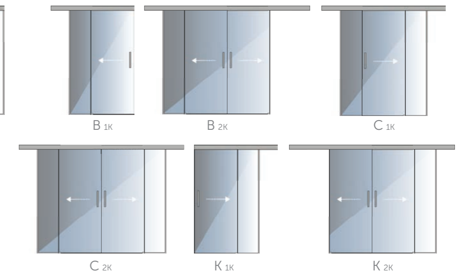
model line GLASS WALLS - SLIDING wall mounted
